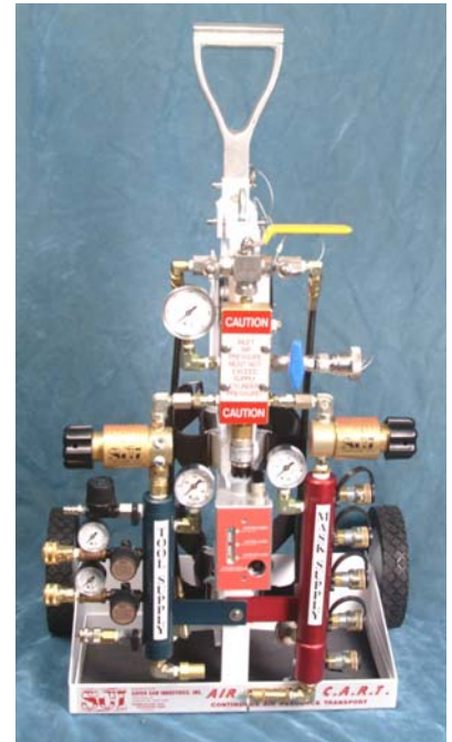
“FDNY” Spec Combi-C.A.R.T. Part # F-ASC-COM-FDN
