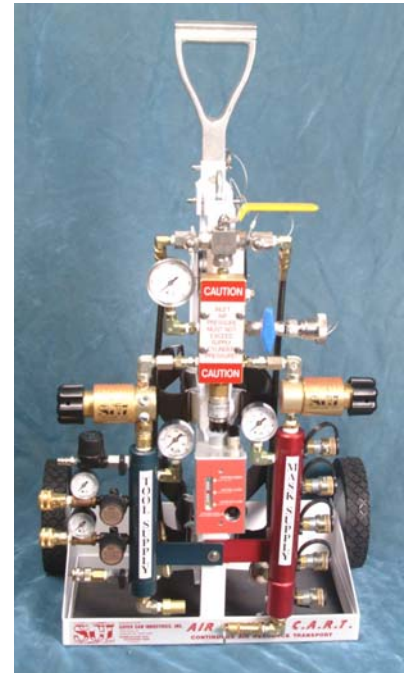
“F” Series Combi-C.A.R.T. Part # F-ASC-COM-001
